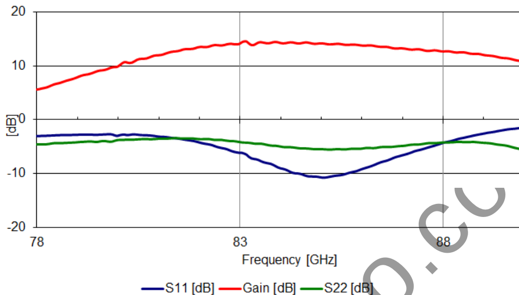
W-MPA 78-90 10 18 - Gain and Return Loss Performance
